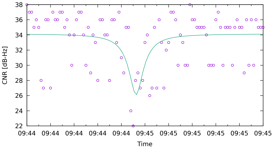
CNR fit for C27 on HuaweiP40 - drive 15 (DOY262)
