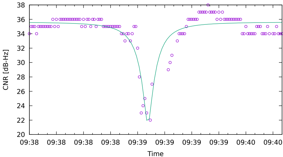
CNR fit for G01 on HuaweiP40 - drive 12 (DOY262)
