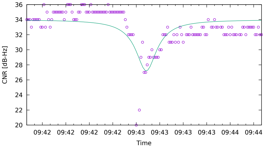
CNR fit for G01 on HuaweiP40 - drive 14 (DOY262)
