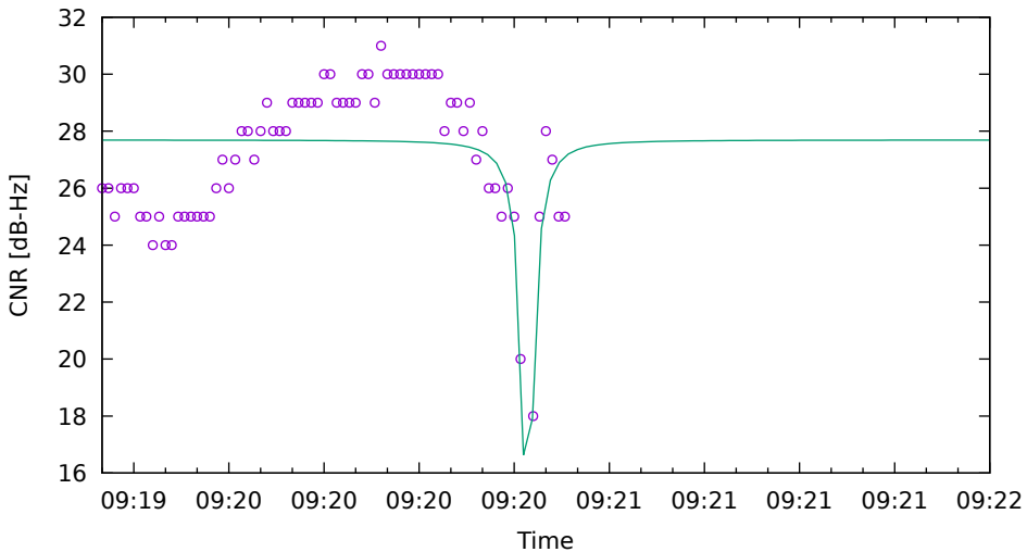
CNR fit for G01 on HuaweiP40 - drive 3 (DOY262)
