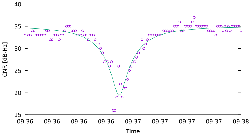
CNR fit for G03 on HuaweiP40 - drive 11 (DOY262)
