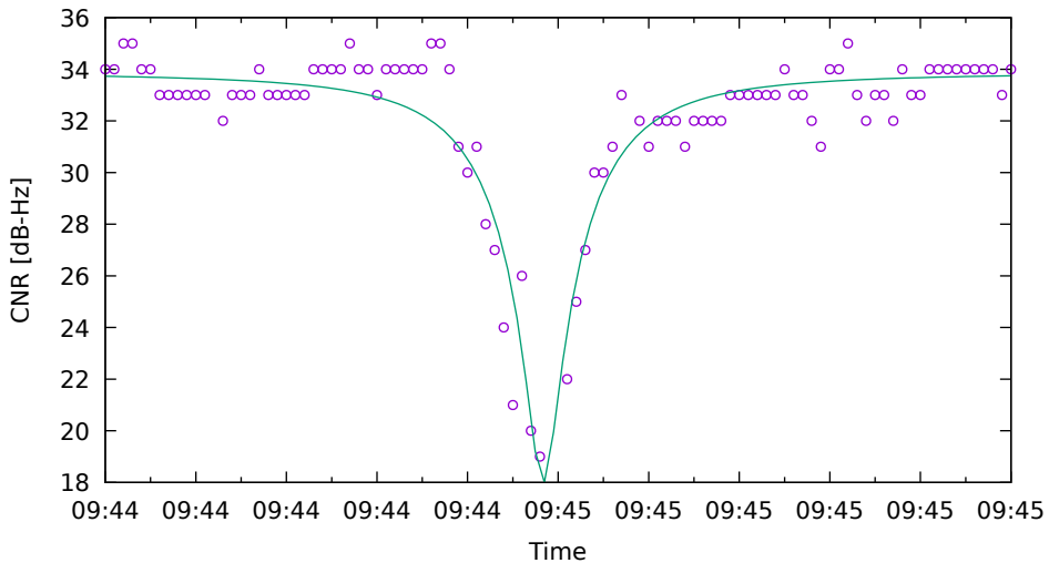
CNR fit for G03 on HuaweiP40 - drive 15 (DOY262)
