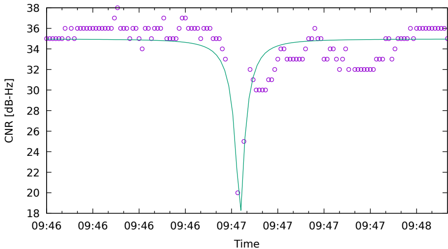
CNR fit for G03 on HuaweiP40 - drive 16 (DOY262)
