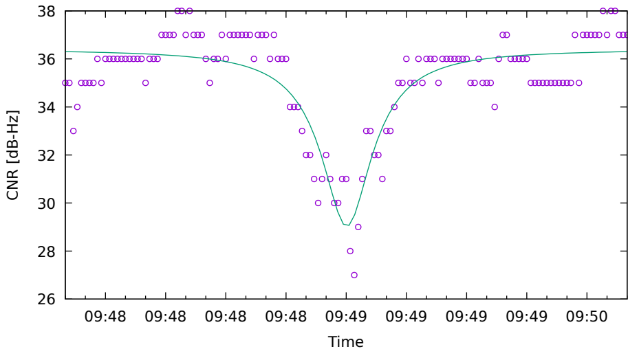
CNR fit for G03 on HuaweiP40 - drive 17 (DOY262)
