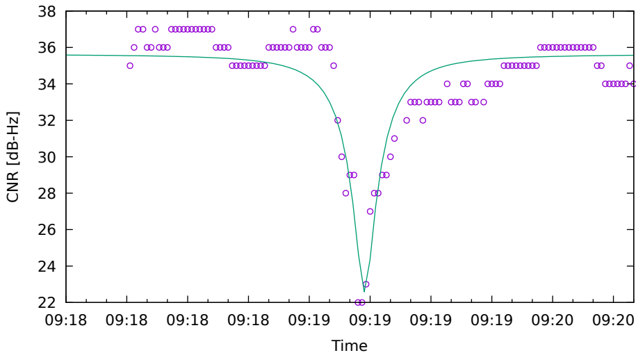
CNR fit for G03 on HuaweiP40 - drive 2 (DOY262)
