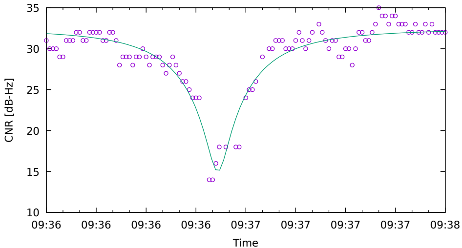
CNR fit for G04 on HuaweiP40 - drive 11 (DOY262)
