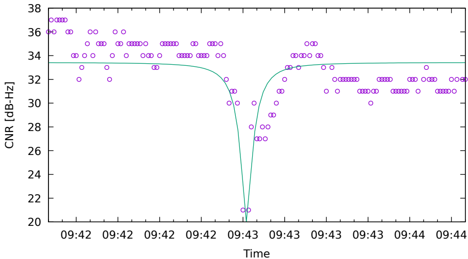
CNR fit for G04 on HuaweiP40 - drive 14 (DOY262)
