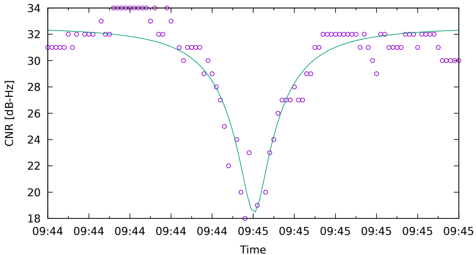
CNR fit for G04 on HuaweiP40 - drive 15 (DOY262)
