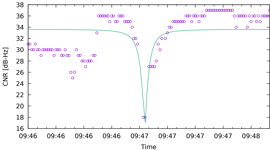
CNR fit for G04 on HuaweiP40 - drive 16 (DOY262)
