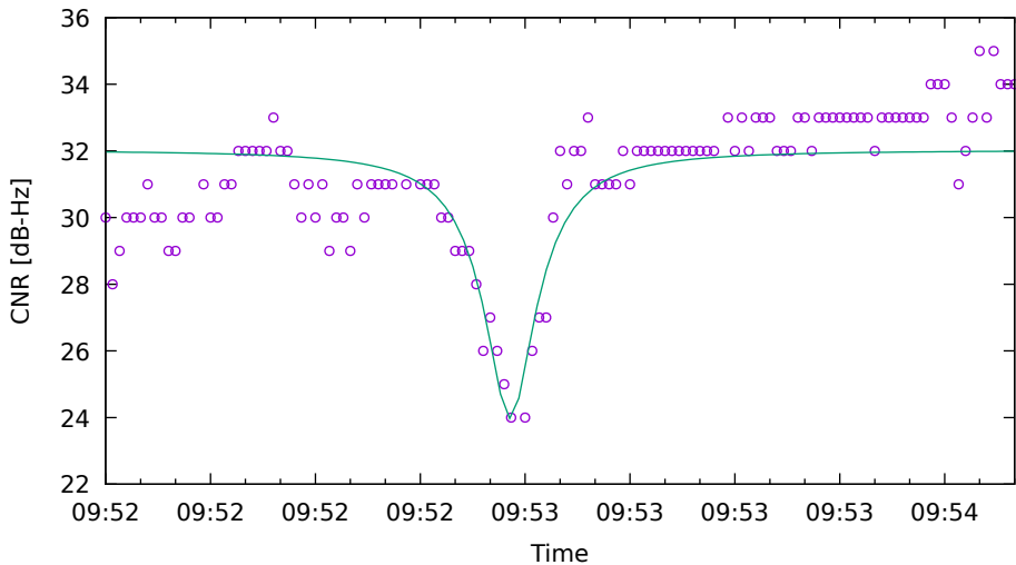
CNR fit for G04 on HuaweiP40 - drive 19 (DOY262)
