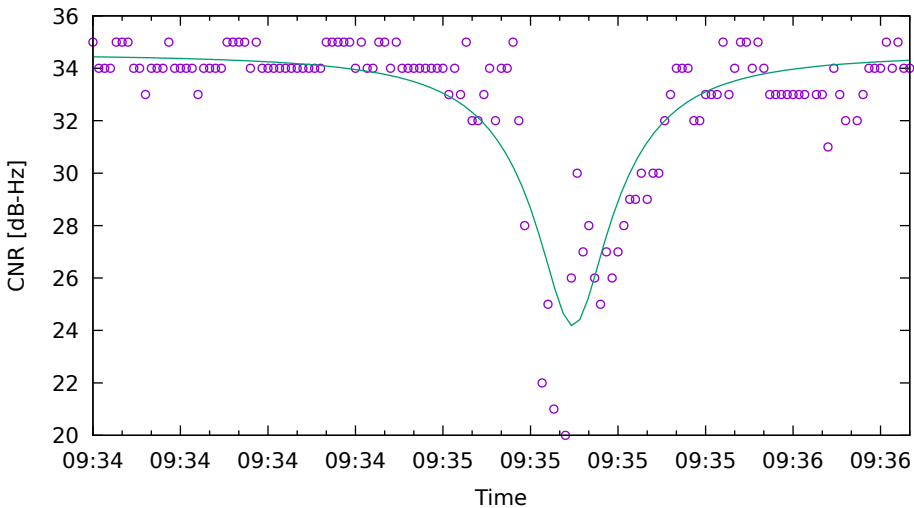
CNR fit for G17 on HuaweiP40 - drive 10 (DOY262)
