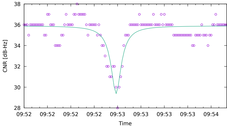
CNR fit for G17 on HuaweiP40 - drive 19 (DOY262)
