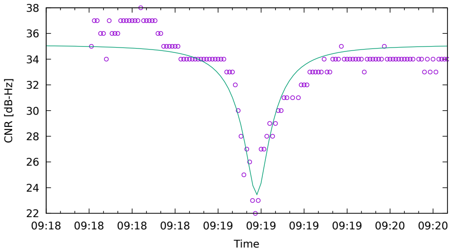
CNR fit for G17 on HuaweiP40 - drive 2 (DOY262)
