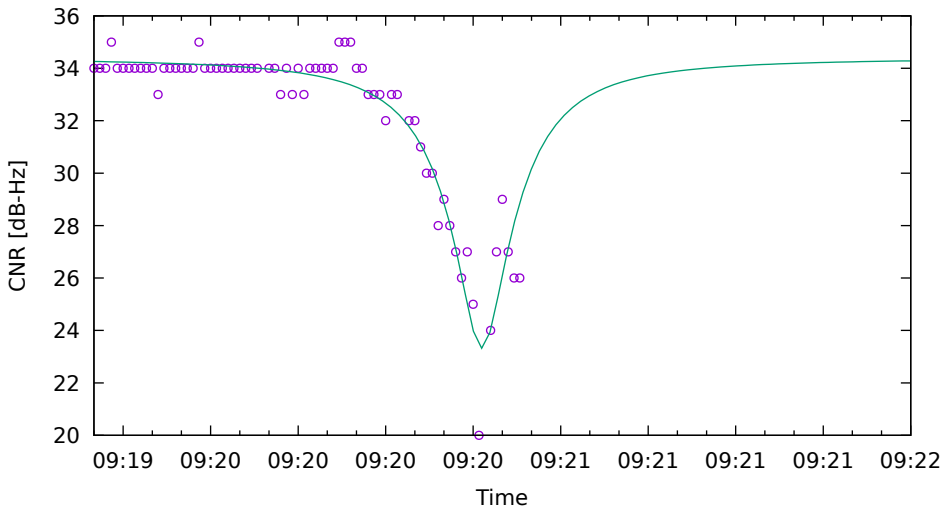
CNR fit for G17 on HuaweiP40 - drive 3 (DOY262)
