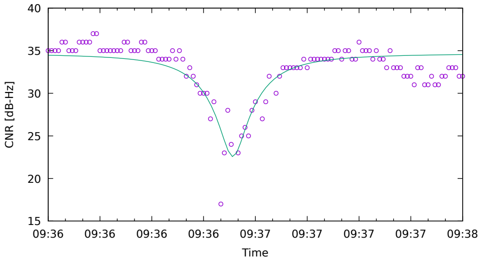
CNR fit for G19 on HuaweiP40 - drive 11 (DOY262)
