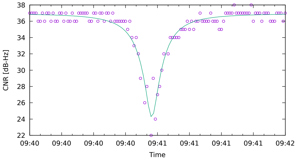
CNR fit for G19 on HuaweiP40 - drive 13 (DOY262)
