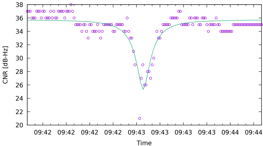
CNR fit for G19 on HuaweiP40 - drive 14 (DOY262)
