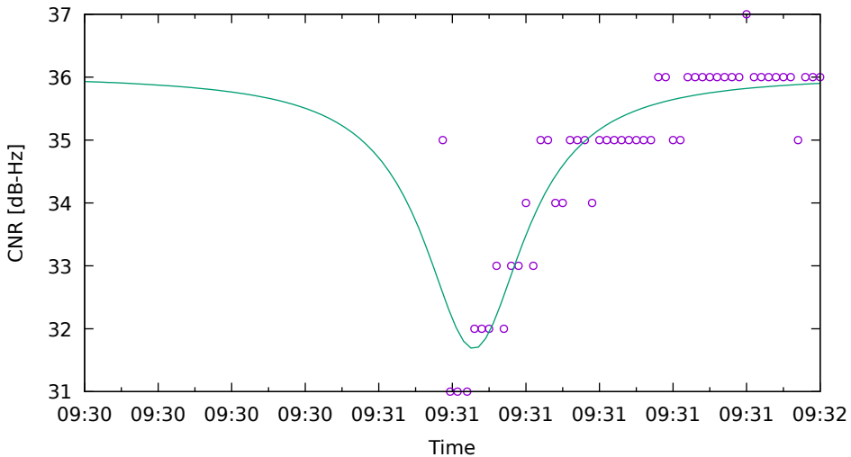
CNR fit for G19 on HuaweiP40 - drive 8 (DOY262)
