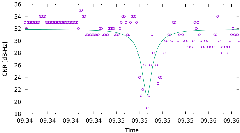
CNR fit for G21 on HuaweiP40 - drive 10 (DOY262)
