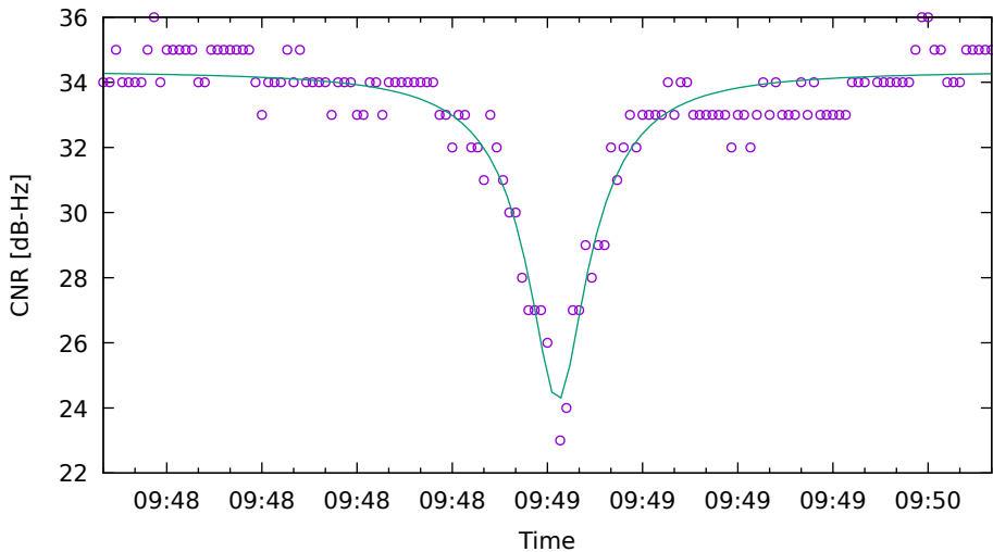
CNR fit for G21 on HuaweiP40 - drive 17 (DOY262)
