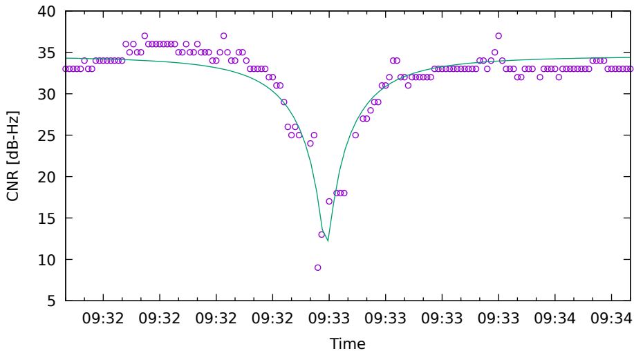
CNR fit for G21 on HuaweiP40 - drive 9 (DOY262)
