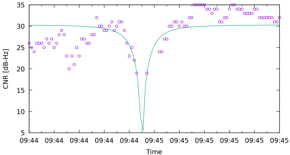
CNR fit for G22 on HuaweiP40 - drive 15 (DOY262)
