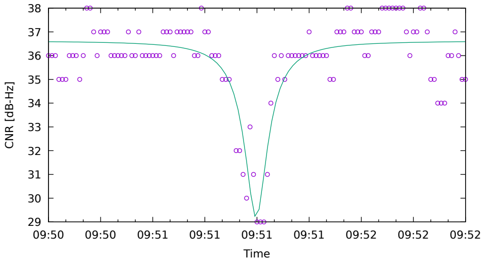
CNR fit for G22 on HuaweiP40 - drive 18 (DOY262)
