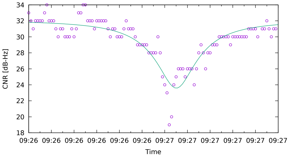
CNR fit for G22 on HuaweiP40 - drive 6 (DOY262)
