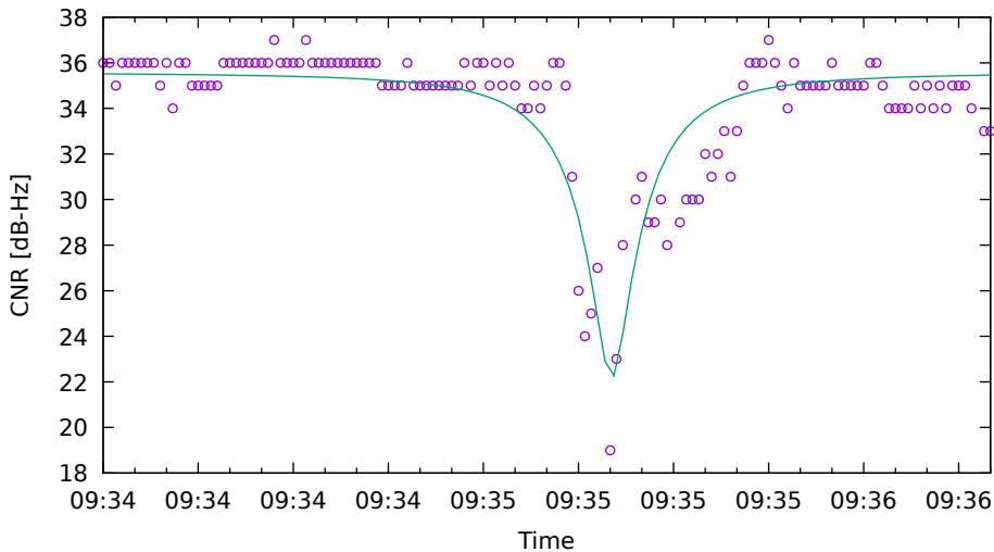
CNR fit for G31 on HuaweiP40 - drive 10 (DOY262)
