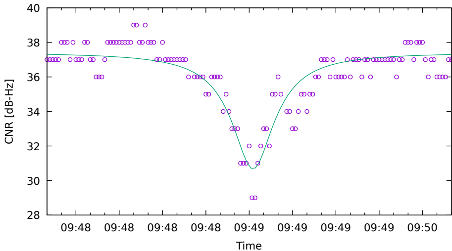
CNR fit for G31 on HuaweiP40 - drive 17 (DOY262)
