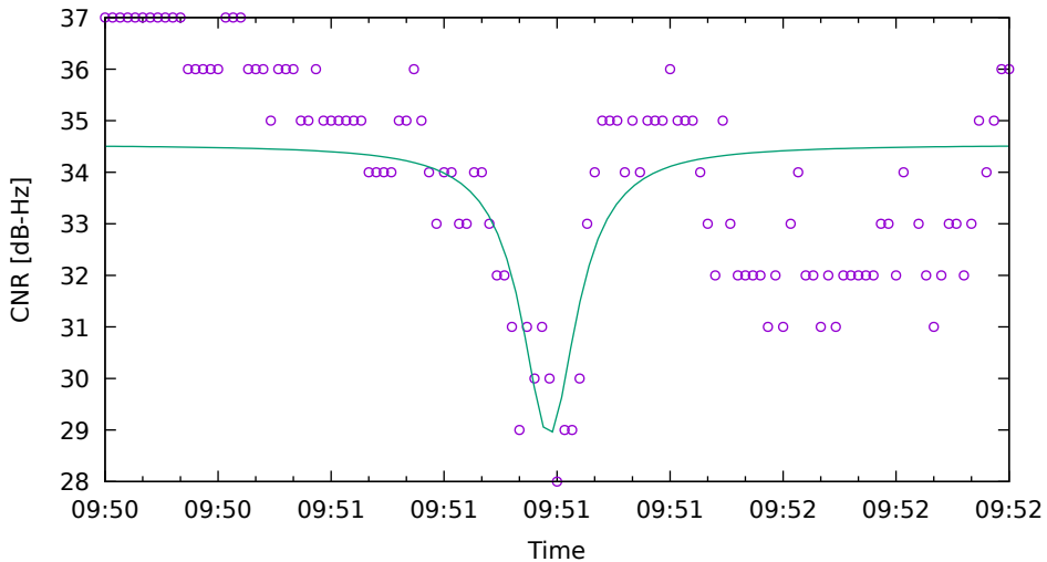
CNR fit for G31 on HuaweiP40 - drive 18 (DOY262)
