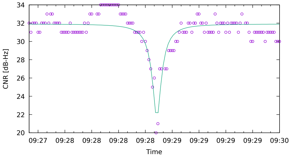
CNR fit for G31 on HuaweiP40 - drive 7 (DOY262)
