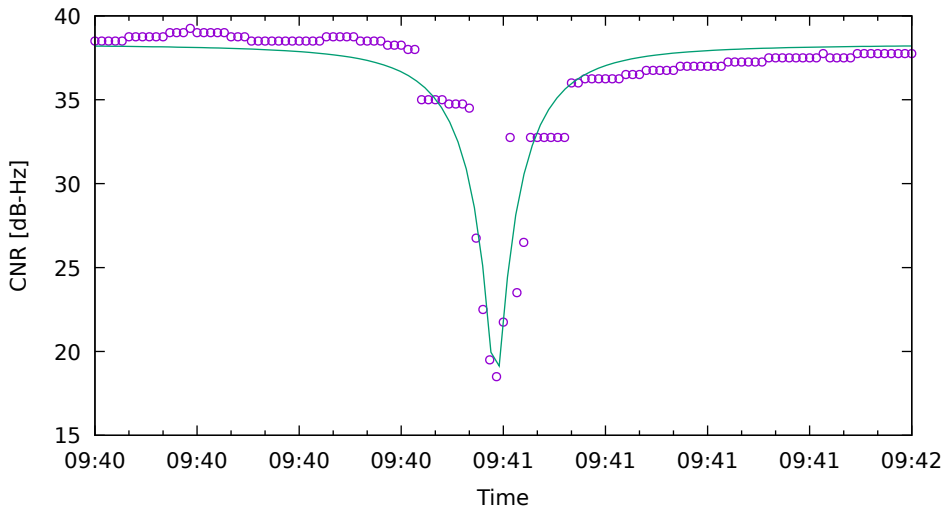
CNR fit for E04 on Xiaomi11T - drive 13 (DOY262)
