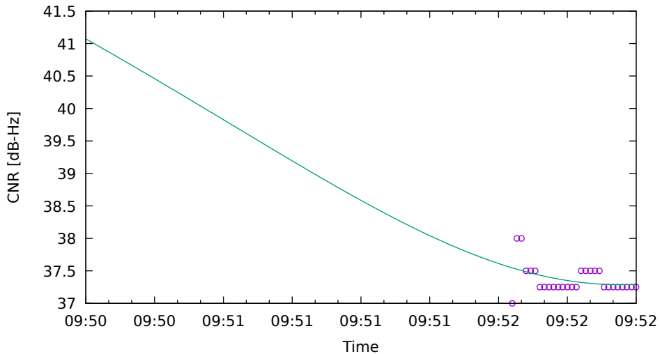
CNR fit for E04 on Xiaomi11T - drive 18 (DOY262)
