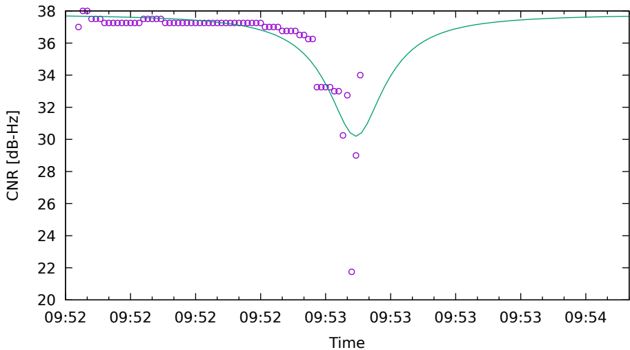
CNR fit for E04 on Xiaomi11T - drive 19 (DOY262)
