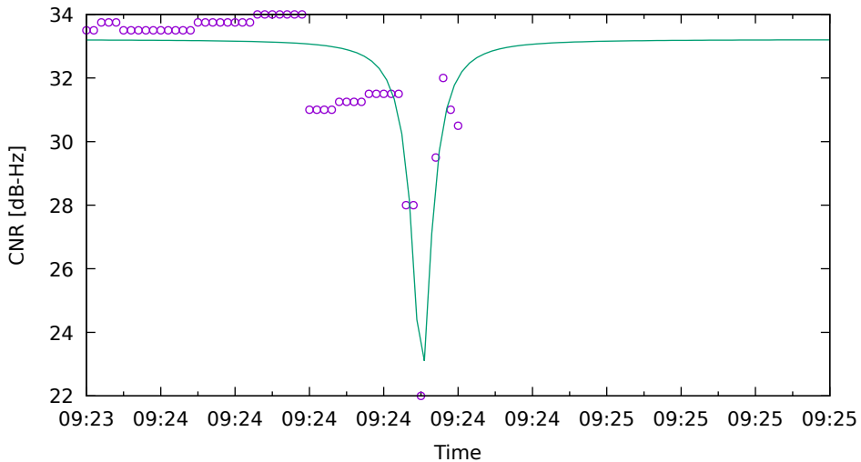
CNR fit for E04 on Xiaomi11T - drive 5 (DOY262)
