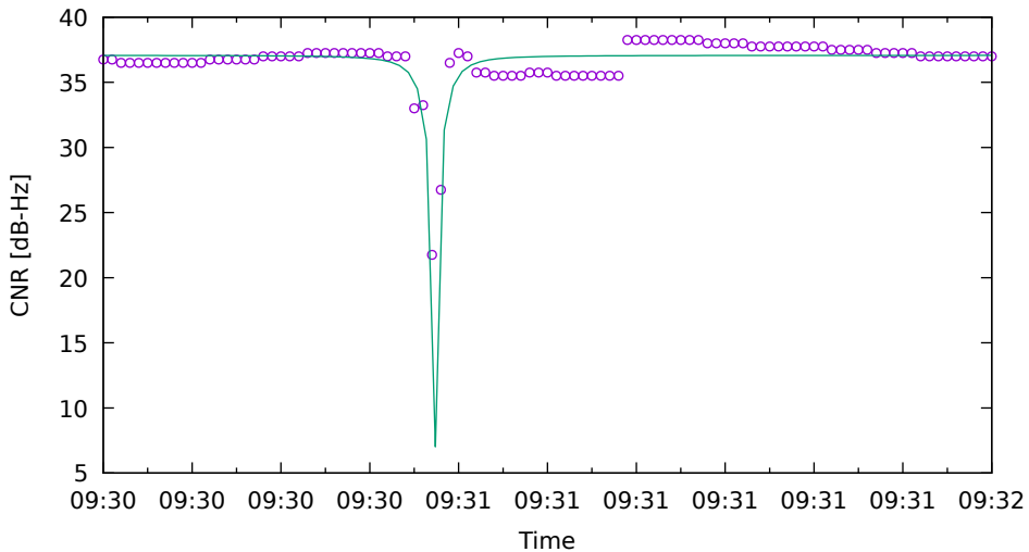
CNR fit for E04 on Xiaomi11T - drive 8 (DOY262)
