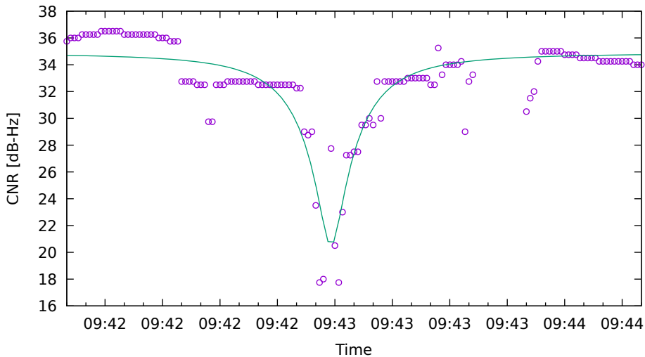
CNR fit for E05 on Xiaomi11T - drive 14 (DOY262)
