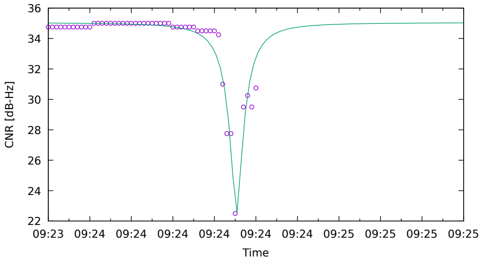
CNR fit for E05 on Xiaomi11T - drive 5 (DOY262)
