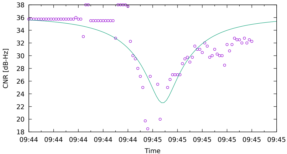
CNR fit for E09 on Xiaomi11T - drive 15 (DOY262)
