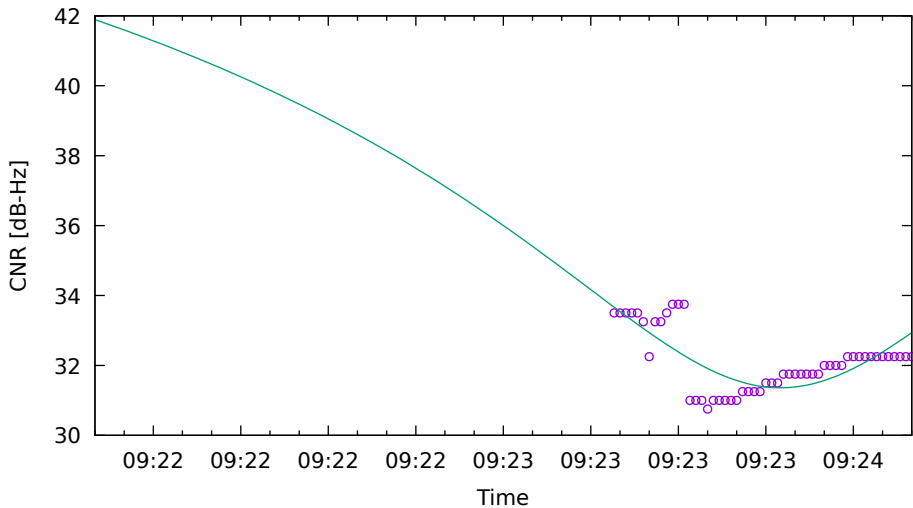
CNR fit for E09 on Xiaomi11T - drive 4 (DOY262)
