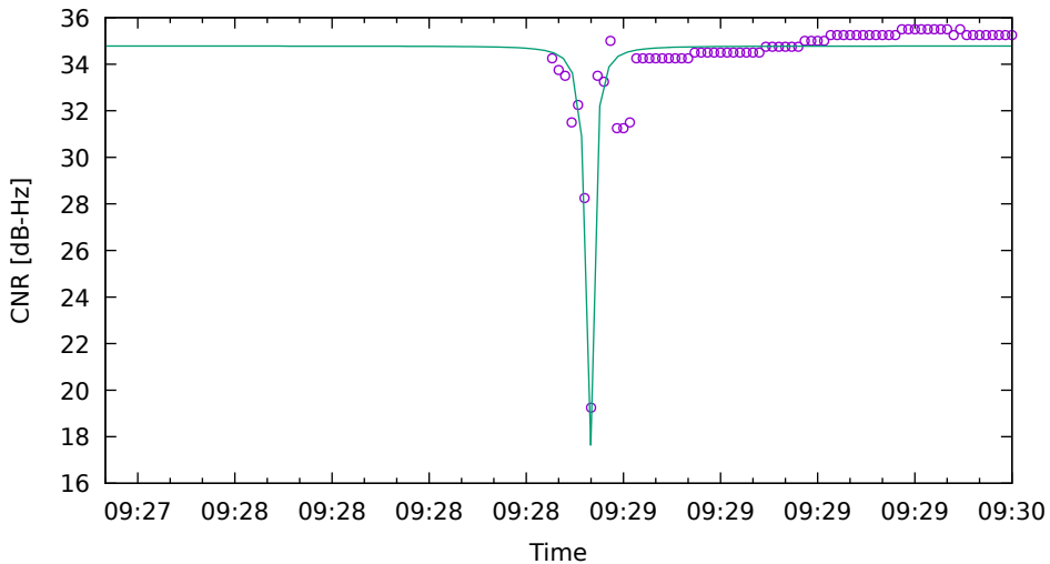
CNR fit for E09 on Xiaomi11T - drive 7 (DOY262)
