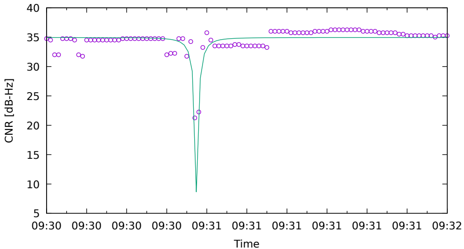
CNR fit for E09 on Xiaomi11T - drive 8 (DOY262)
