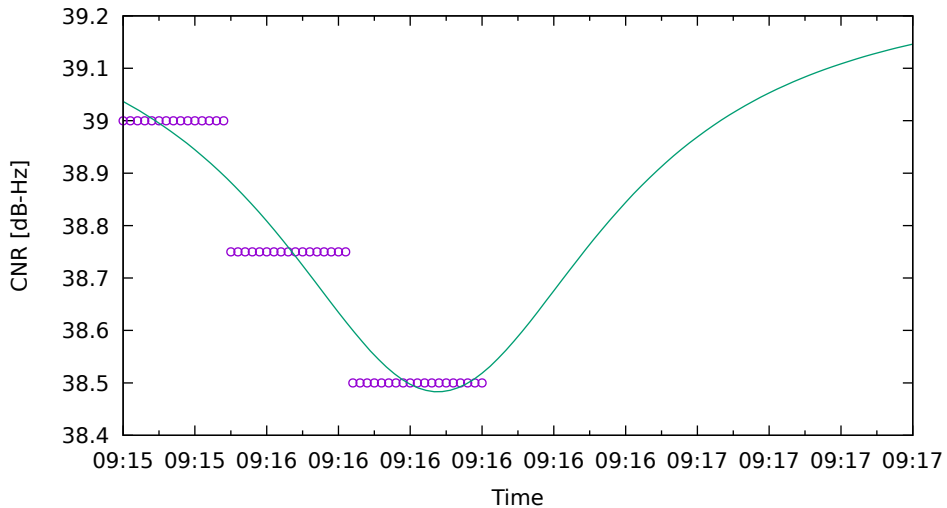
CNR fit for E34 on Xiaomi11T - drive 1 (DOY262)
