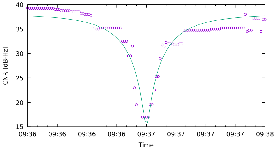
CNR fit for E34 on Xiaomi11T - drive 11 (DOY262)
