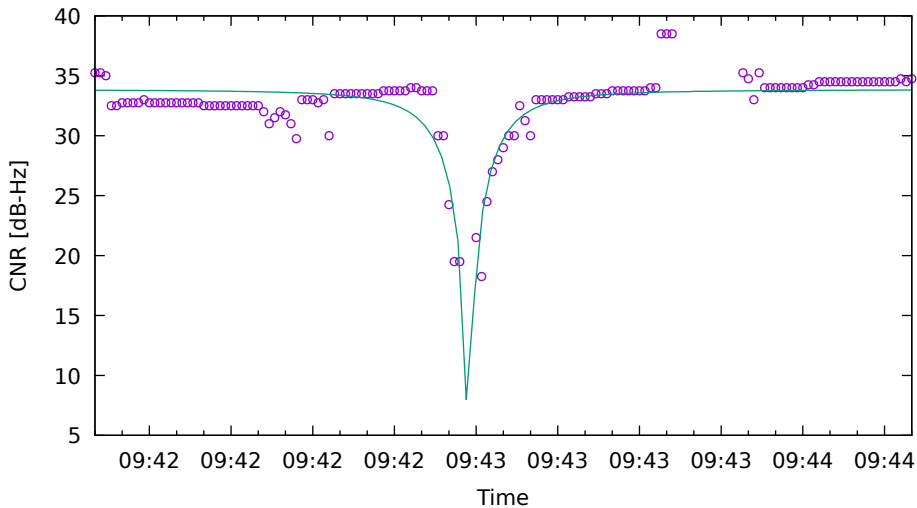
CNR fit for E34 on Xiaomi11T - drive 14 (DOY262)
