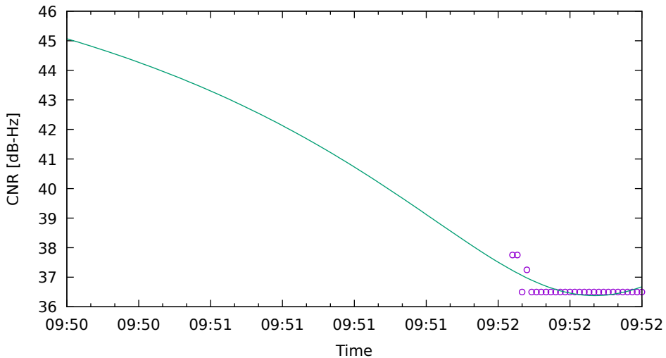
CNR fit for E34 on Xiaomi11T - drive 18 (DOY262)
