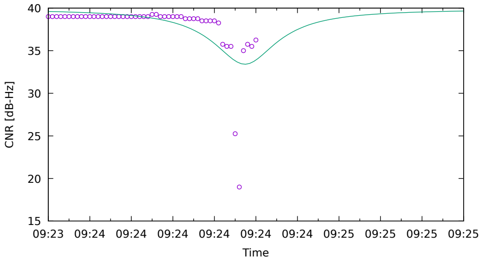
CNR fit for E34 on Xiaomi11T - drive 5 (DOY262)
