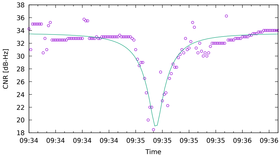
CNR fit for E36 on Xiaomi11T - drive 10 (DOY262)
