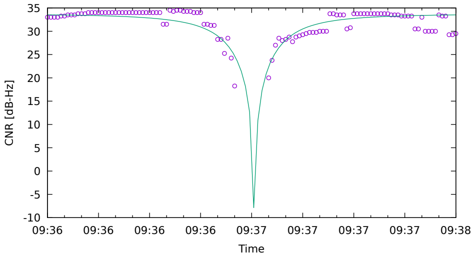
CNR fit for E36 on Xiaomi11T - drive 11 (DOY262)
